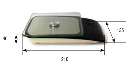
Dimensions (mm)
